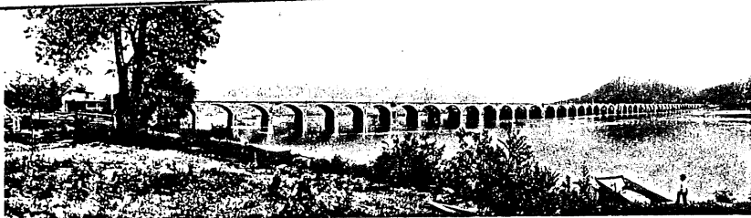
The P. R. R. Bridge over the Susquehanna River. The longest stone bridge in the world, 3800 feet long, 52 feet wide, 48 arches and 440,000,000 pounds of stone
